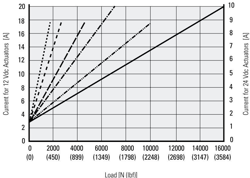
Load vs. Current
