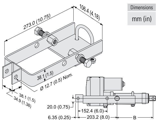
PPA Rear Clevis Mounting Kit - Type 2
