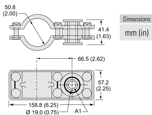
Electrak PPA Tube Mount - Light Duty 3330 N (750 lbf)
