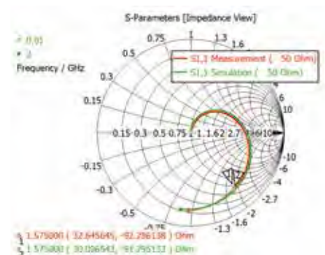
Comparison of simulation and measurement: The transformation shown in the Smith chart
