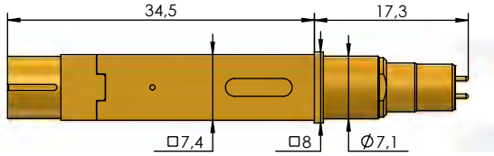
Connection for Plug SE-819-V2
