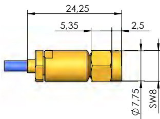
PC3.5-m (straight)
