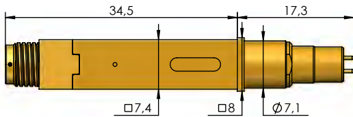
Connection for screw-in Plug SE-819-V2
