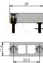
HAS-819 D8-160 (Consisting of Contact Mounting, Threaded Pins, Springs and Screws)
