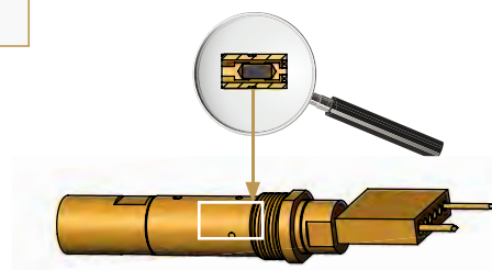
HFS with integrated Filter Example: HFS-440 007 051 A 4807 P5-AS 4M
