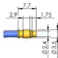
MMPX™-m (straight)
