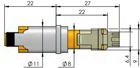
Connection for USB-Mini Plug
