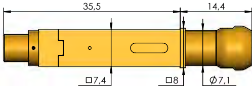
Connection for Screw Plug SE-819-V2
