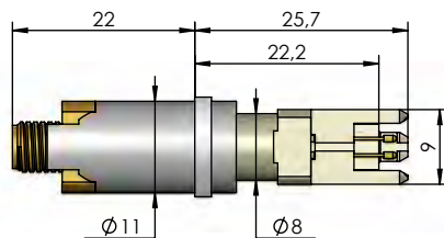
Connection for Screw-in Plug SE-821 MX49
