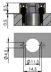
Customizing recommendation for Mounting Plate
