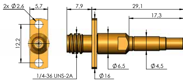
Connection for SMA Plug
