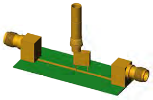
Example of test set-up with three-port measurement
