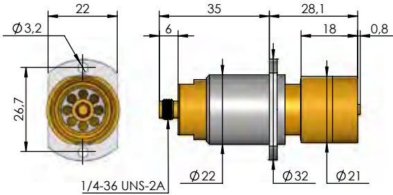
Connection for SMA Plug
