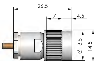
PC3.5-m (straight)
