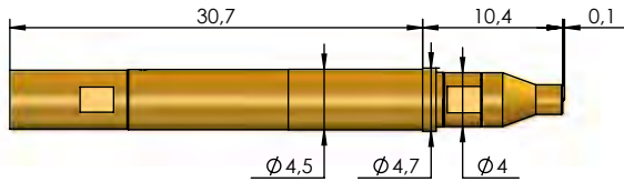
Connection for MMPX Plug
