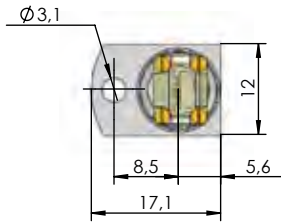
Connection for USB-Mini Plug
