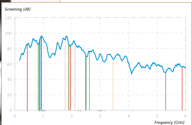
Screening attenuation in the RF range of up to 6 GHz
